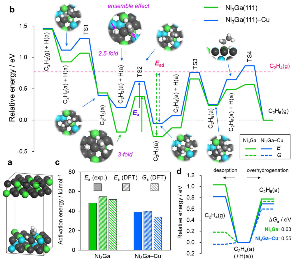
Fig. 4 DFT calculations for acetylene hydrogenation. (a) Example of the optimized structure in the slab model: \text{C}_2\text{H}_2(\text{a}) + \text{H}(\text{a}) on \text{Ni}_3\text{Ga}(\text{111})\text{-Cu} . (b) Energy landscapes of the stepwise hydrogenation from acetylene to ethane. Sum of the bare slab and gas-phase \text{C}_2\text{H}_6 was set to zero in energy. (c) Comparison of activation energies. (d) Energy diagrams of ethylene desorption and overhydrogenation.
