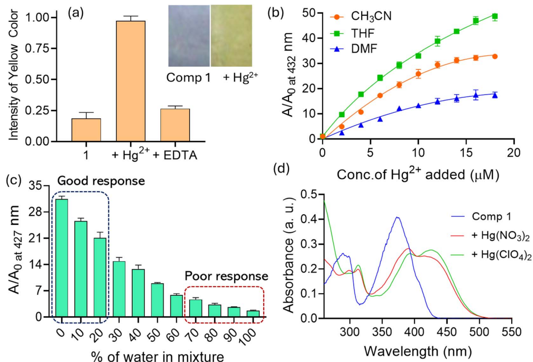
Fig. 5 (a) Reusable paper strips (coated with compound 1 ) for detection of \text{Hg}^{2+} ions. (b) Changes in absorbance of 1 (10 \mu\text{M} ) upon addition of \text{Hg}^{2+} (0–20 \mu\text{M} ) in different organic media. (c) Changes in absorbance at the 427 nm band with \text{Hg}^{2+} ions in different \text{CH}_3\text{CN} – \text{H}_2\text{O} mixtures. (d) UV-vis spectra of 1 (10 \mu\text{M} ) with different \text{Hg}^{2+} salts (25 \mu\text{M} ) in a \text{CH}_3\text{CN} medium [each experiment was independently performed three times for reproducibility].
