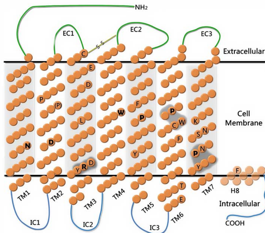
Fig. (1). General scheme of topology and location of conserved residues in Rhodopsin-like GPCRs. Number of residues and their locations in each TM is based on chemokine receptor CXCR4 (H8 is not present in the crystal structure so it is shown transparent). Residues in bold are the most conserved in each TM. Sequence motifs are shown as gray areas. An alternative position of proline residue in TM2 is denoted by (P). Detailed description of figure is done in main text.
