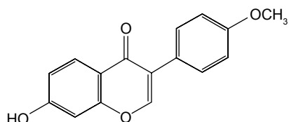
Figure 1 Chemical structural of 7-hydroxy-4'-methoxyisoflavone (formononetin).
