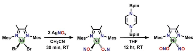
Scheme 2 Synthesis of (DIM)Ni(NO x ) 2 complexes, as well as the synthesis of (DIM)Ni(NO)(ONO) from (DIM)Ni(NO 2 ) 2 . The bis-nitrate and bis-nitrite complexes are O-bound and bidentate in the solid-state molecular structures (Fig. 1), we have drawn them as monodentate here for simplicity.
