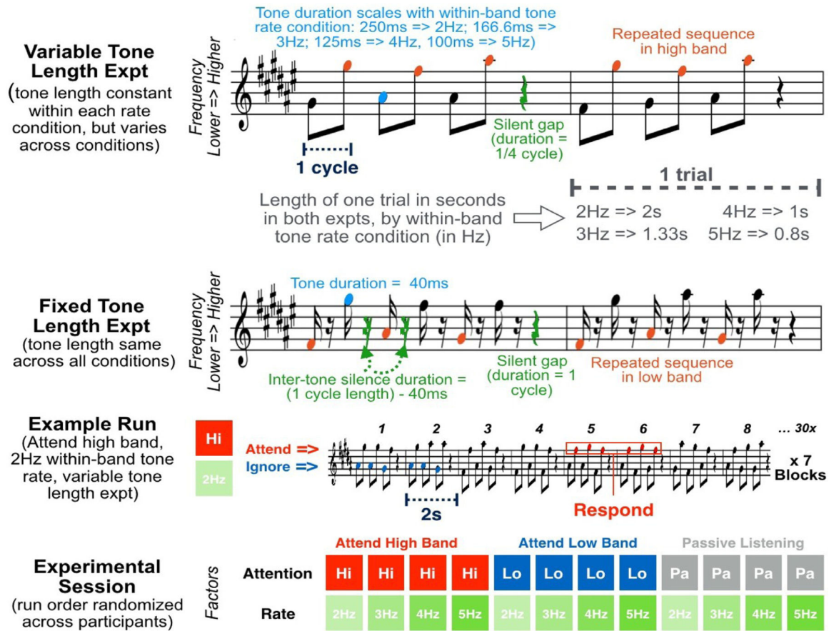
Fig. 2. Schematics showing experimental design. The top row shows two trials of the Variable Tone Length Experiment, and the second row two trials of the Fixed Tone Length Experiment, in quasi-musical notation. For ease of depiction on one staff, fundamental frequencies depicted by musical notes are one octave higher than those used in the experiment. For each tone rate condition in the variable tone length experiment, all tones are set to a condition-specific duration (see Figure and Methods); in the fixed tone length experiment, all tones are 40 ms long regardless of rate condition. The third row shows a segment of an example run of the 'attend high band, 2 Hz within-band tone presentation rate' condition from the variable tone length experiment. Each run is made up of 7 blocks of 30 trials, where a trial contains two interleaved 3-tone sequences, one in the higher frequency band, and one in the lower band. There are three low/high-tone 'cycles' in a trial, followed by a silence equal in duration to an additional cycle. The bottom row shows all twelve runs for a single experiment, where each run is a combination of attention condition and within-band tone presentation rate. Note that run order is randomized across participants. See supplementary material for audio of example blocks.
