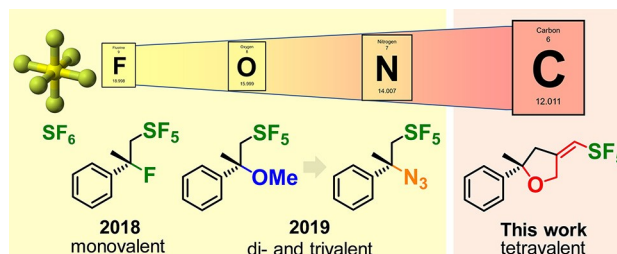
Figure 1. The recent advancement of photoredox catalytic methods to convert SF_6 into pentafluorosulfanylated organic compounds as valuable synthesis building blocks.
