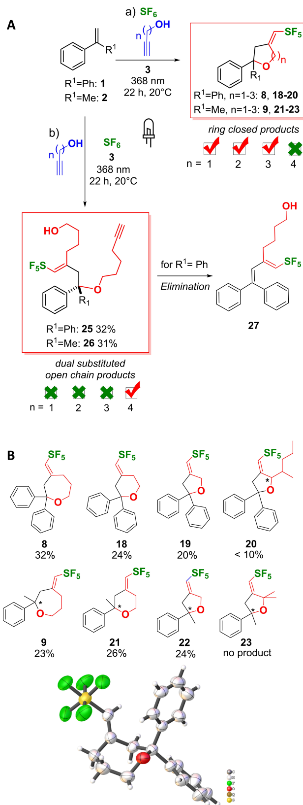
Figure 5. A: Overview of reactions: a) 0.20 mmol 1 or 2 (0.2 M in MeCN), 20.0 equiv. 1-alkynol, 10 mol% \text{BEt}_3 , 10 mol% 3 , MeCN, 20^\circ\text{C} , 368 nm, 2.8 bar \text{SF}_6 . b) 1.00 mmol 1 or 2 (0.2 M in MeCN), 20.0 eq. 1-hexynol, 10 mol% \text{BEt}_3 , 10 mol% 3 , MeCN, 20^\circ\text{C} , 368 nm, 2.8 bar \text{SF}_6 . B: Substrate scope. Image: XRD structure of the isolated product 8. Volume corrections (alcohol volume) neglected except for optimization process of the lead compound to facilitate the protocol. The yields were determined by ^{19}\text{F} NMR spectroscopy.
