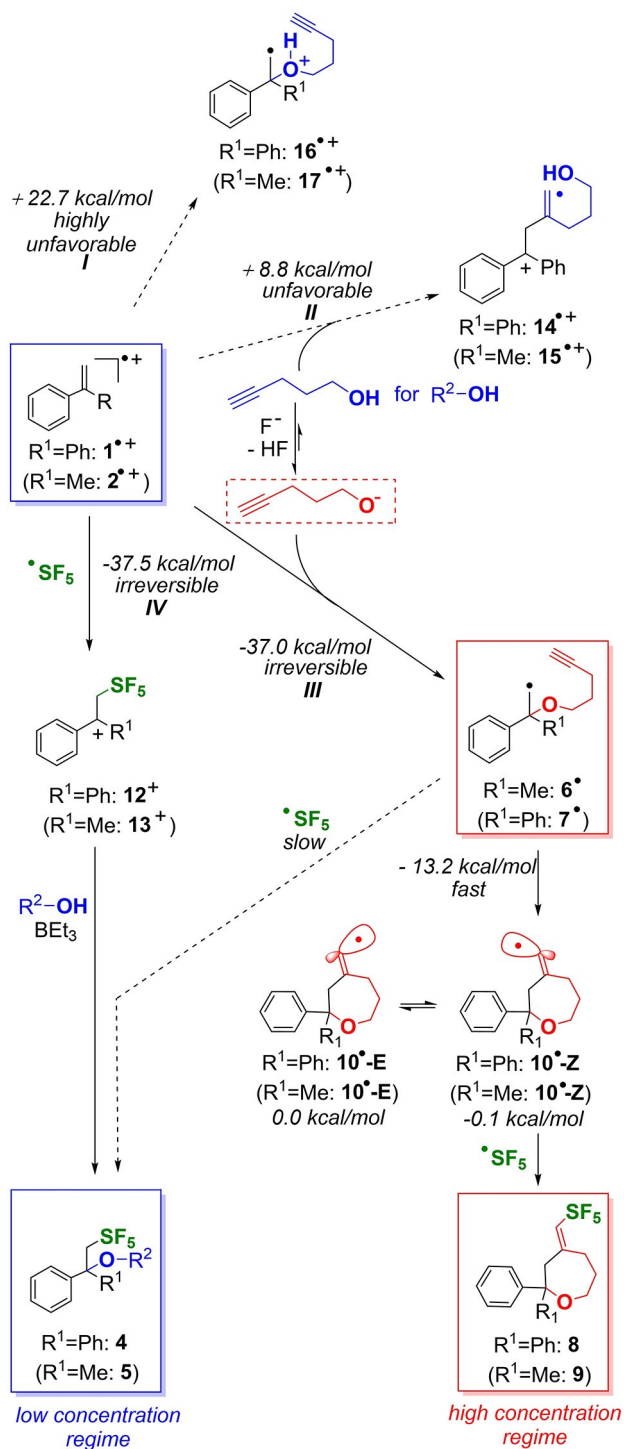
Figure 4. Proposed mechanism controlling the formation of the acyclic products 4 and 5 vs. the ring closed products 8 and 9 during photoredox catalytic pentafluorosulfanylation of substrates 1 and 2, respectively, in the presence of 1-pentynol. Geometry optimizations and frequency calculations: DFT/def2-TZVP/M06-2X, 293 K, CPCM (MeCN). Refinement of electronic energies: DLPNO-CCSD(T)/def2-TZVP/CPCM (MeCN).
