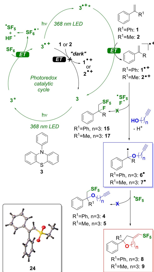
Figure 2. Overview of reaction pathways after photoredox catalytic activation of SF 6 by irradiation at 368 nm and pentafluorosulfanylation of \alpha -methyl ( 1 ) and \alpha -phenyl styrene ( 2 ) with novel intramolecular radical-alkyne addition to cyclization products 8 and 9 . Insert: Structure of the isolated sulfone 24 .
