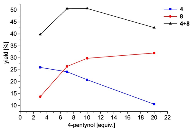
Figure 3. Yields of 4 and 8 and the total yields of both products depending on the concentration of 4-pentynol. The yields were determined by ^{19}\text{F} NMR spectroscopy. Reaction conditions: 0.20 M 1 , 10 mol% \text{BET}_3 , 10 mol% 3 , 22 h, 20 °C, MeCN, 368 nm LED. 2.8 bar \text{SF}_6 .
