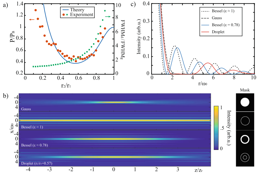
Figure 2. (a) Plot of the ratio between the optical power (for z = 0 ) distributed across the droplet side lobes with respect to the Bessel lobe power as a function of the ratio r_2/r_1 . The solid line is the theoretical prediction while red dots are experimental data. A plot of the ratio between the axial FWHM of the droplet beam and the Gaussian beam as a function of the ratio r_2/r_1 is reported in the same graph. Top-view ( xz plane) (b) and radial (c) intensity profiles of a Gaussian, an ideal Bessel beam ( \epsilon = 1 ) and a short Bessel beam ( \epsilon = 0.78 ) of comparable axial FWHM to that of the droplet beam as a function of the number of Rayleigh lengths and for an equal NA. For r_2/r_1 \sim 0.57 , the light distributed across the droplet side lobes is about 62% and 48% lower than that of an ideal and a short Bessel beam respectively. Associated beam amplitude masks (inset).
