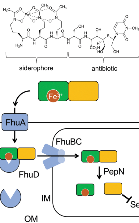
Fig. 5 Albomycin enters a bacterial cell using the bacterial iron uptake system. The siderophore unit is important for the compound to get into bacterial cells by utilizing the bacterial iron uptake system. First, the ferric siderophore passes the outer membrane through the ferrichrome outer membrane transporter FhuA. In the periplasm, the ferrichrome binds FhuD, which is then transported into the cytoplasm through the membrane channel FhuBC. In the cytoplasm, the amide bond is hydrolysed by the endogenous peptidase PepN releasing the active thioheptose nucleoside unit, which inhibits seryl-tRNA synthetase (SerRS). OM, outer membrane; IM, inner membrane.
