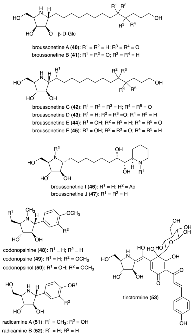
Fig. 9 Chemical structures of plant-derived N -ribomimetics.
