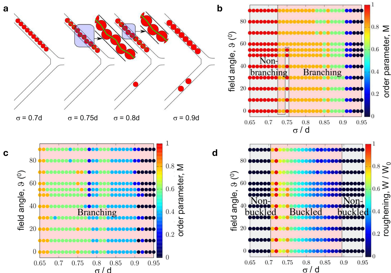
Fig. 4 | Buckling during branching at the Y-junction. a Simulation snapshots ( \vartheta = 0^\circ ) showing the transition between the buckled and non-buckled states and the splitting induced by varying the normalized particle size \sigma/d . Buckling is highlighted in the top insets for \sigma = 0.75d and \sigma = 0.8d , see Supplementary Movie 4. b Order parameter M in the (\sigma/d, \vartheta) plane from numerical simulations. c Branching
