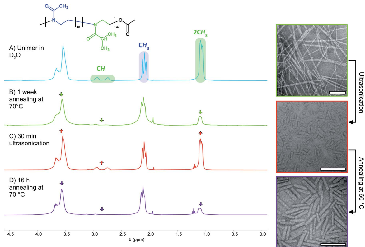
Fig. 3 Concomitant nanofibre fragmentation and BCP dissolution. Left, ^1\text{H} NMR spectra (400 MHz, 2 \text{ mg mL}^{-1} in \text{D}_2\text{O} ) of \text{PMeOx}_{48}\text{-}b\text{-PiPrOx}_{47} unimer (A), nanofibres prepared annealing the BCP solution at 70^\circ\text{C} for 1 week (B), a mixture of seed fragments and BCP unimer prepared via ultrasonication (C) and elongated seeds (D). Right, TEM images showing polydisperse nanofibres (top), seeds (middle) and elongated seeds (bottom). Scale bars equal to 250 nm.
