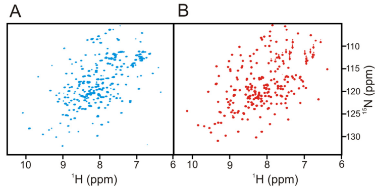
Fig 4. NMR spectra of yeast Adk1 and E. coli Adk. (A) ^1\text{H} - ^{15}\text{N} HSQC spectrum of Adk 1 yeast (B) ^1\text{H} - ^{15}\text{N} HSQC spectrum of Adk eco . The spectra were acquired at 20°C and show that both enzymes are properly folded at the conditions used in this study.
