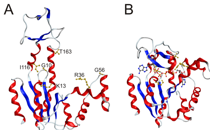
Fig 1. Structural dynamics in \text{Adk}_{\text{eco}} and positions of mutations. (A) Structure of the open and substrate free conformation of \text{Adk}_{\text{eco}} [16] (4AKE.pdb). Positions mutated in this study are indicated with ball and stick representations and colored in gold. (B) Crystallographic structure of \text{Adk}_{\text{eco}} in the closed and active conformation [17] (1AKE.pdb). The inhibitor Ap5A [29] is displayed with a ball and stick representation.
