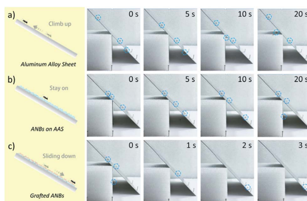
Fig. 4 The insect anti-adhesive performance of grafted ANBs. Pheidole jucunda ants crawling on (a) AAS, (b) HD-ANBs and (c) Grafted HD-ANBs.
