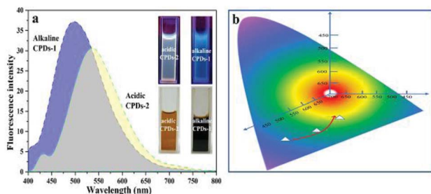
Fig. 1 (a) The fluorescence emission spectra (Ex = 405 nm), fluorescence imaging under UV light (Ex = 365 nm,) and apparent performance of the CPDs-1 and CPDs-2 water solutions. (b) The gradually varying fluorescence palette.
