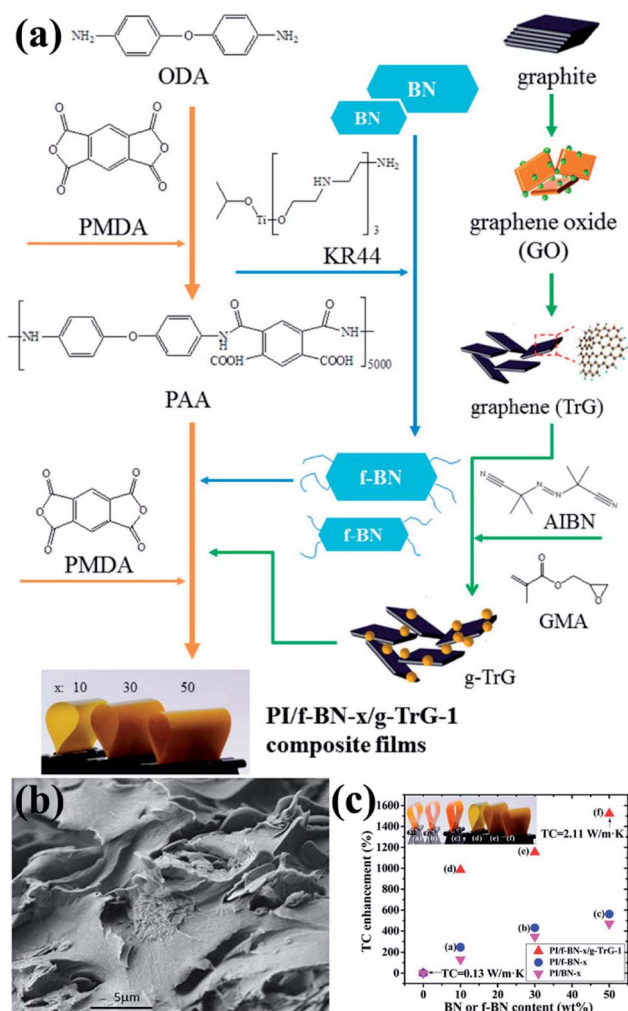
Fig. 18 (a) Preparation of fillers (f-BN and g-TrG) and composite films (PI/f-BN-x/g-TrG-1). (b) SEM observation of the fractured surface of PI/f-BN-30/g-TrG-1. (c) Variations in thermal conductivity with BN or f-BN contents. Reproduced with permission from ref. 123.
