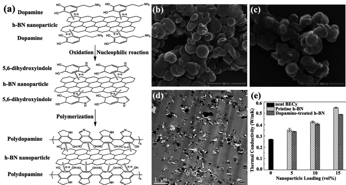
Fig. 5 (a) Illustration of polydopamine functionalized h-BN. SEM observations of h-BN (b) and dopamine-treated h-BN (c). (d) TEM image of h-BN/BECy composite with 15 vol% dopamine-treated h-BN. (e) Variations in the thermal conductivity of h-BN/BECy composite with nanoparticle loadings. Reproduced with permission from ref. 73.
