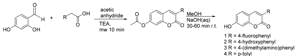
Scheme 1. General Procedure for the Synthesis of Coumarin Derivatives
