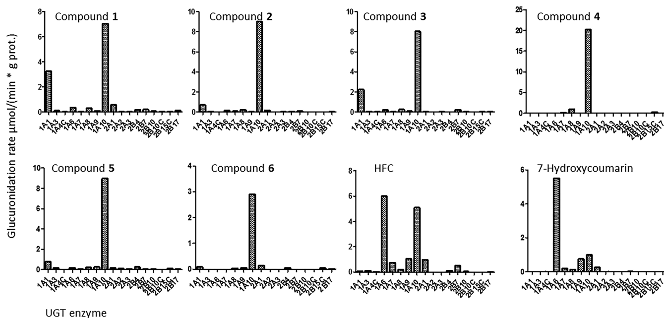
Figure 5. Glucuronidation of C3-substituted 7-hydroxycoumarins by human UGTs. Glucuronidation was determined at 10 \mu\text{M} aglycone concentration.
