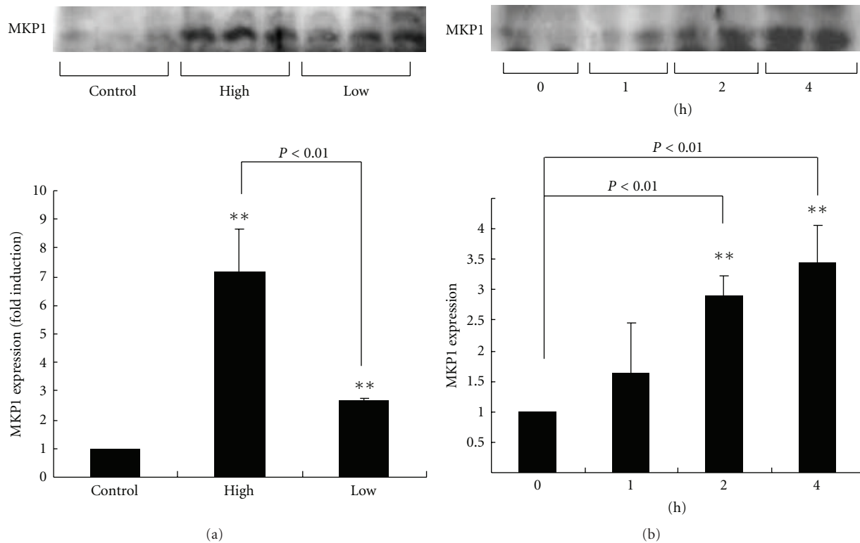
FIGURE 3: Induction of MKP1 by high frequency of GnRH pulse stimulation. (a) LbT2 cells were stimulated with vehicle (control) or pulsatile GnRH (10 nM, 5 min pulse flow per each pulse) at a frequency of one pulse every 30 min (high) or one pulse every 2 h (low). After 16 h stimulation, MKP1 protein expression was determined by Western blotting. MKP1 expression was increased predominantly following high rather than low-frequency GnRH pulse stimulation. (b) Time course of MKP1 expression following high-frequency GnRH pulse. Under the high frequency GnRH pulse stimulation, MKP1 protein expression was observed clearly at 2 h after the start of pulse stimulation (four GnRH pulses). ** P < 0.01 versus control [26].
