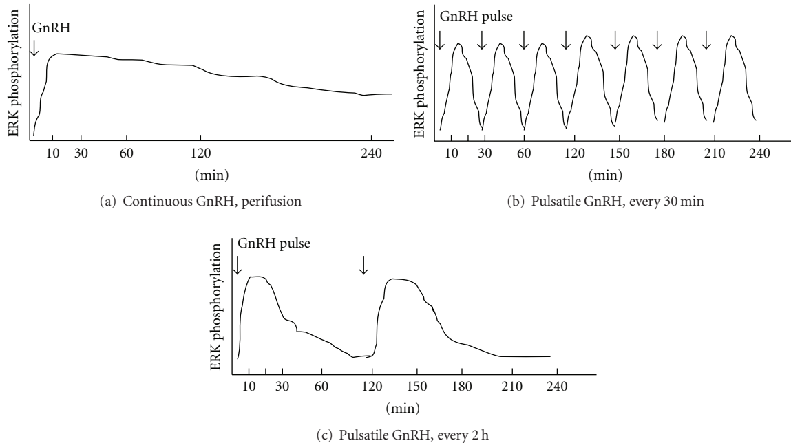
FIGURE 2: Schematic pattern of ERK activation by perifused GnRH stimulation. (a) When cells were exposed to continuous GnRH in perfused conditions, ERK activation was significantly increased, after 10 min, and increased ERK phosphorylation was sustained and gradually decreased to the basal. (b) At high frequency of GnRH pulse stimulation (one pulse every 30 min), ERK phosphorylation increased to a maximum at 10 min, and then levels rapidly decreased to basal levels within 30 min. A similar pattern of ERK phosphorylation was observed in response to subsequent pulse of GnRH. (c) At a slower frequency of GnRH pulse stimulation (one pulse every 2 h), ERK was more rapidly phosphorylated by GnRH pulse, and increase was more sustained, remaining elevated, and then slowly decreased to the baseline levels. A similar pattern of ERK phosphorylation was observed in response to subsequent pulse of GnRH.
