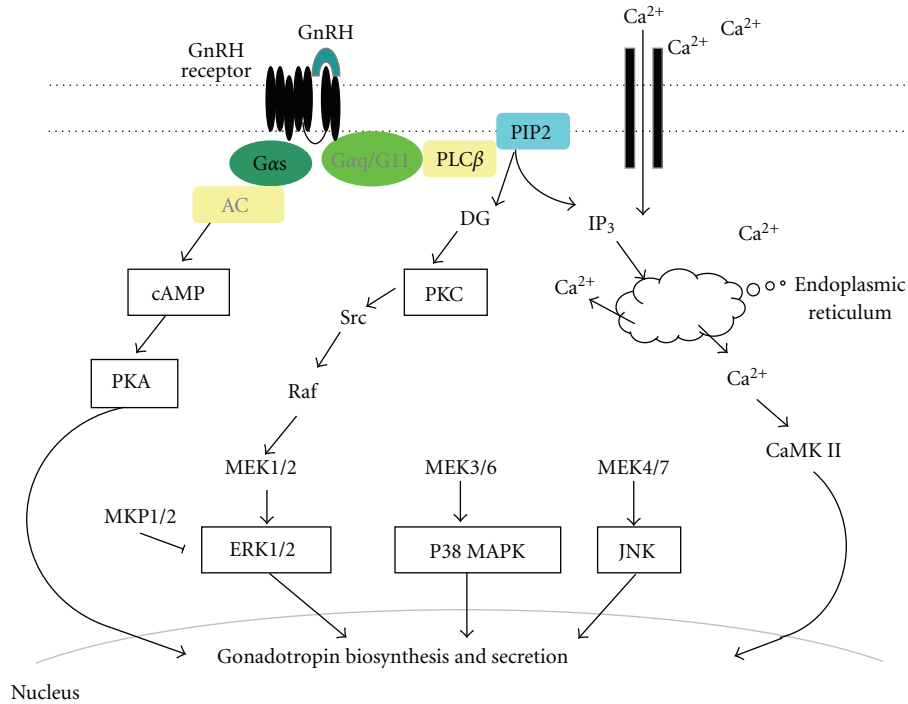
FIGURE 1: Schematic summary of intracellular signaling by GnRH. The initial phase of GnRH action involves Gq-protein-mediated stimulation of phospholipase C \beta (PLC \beta ), leading to the formation of 1,4,5-triphosphate (IP _3 ) and diacylglycerol (DG). IP _3 induces the release of intracellular calcium from endoplasmic reticulum, and DG activates protein kinase C (PKC), which ultimately activates extracellular signal-regulated kinase (ERK). P38 MAPK, c-Jun N-terminal kinase (JNK), and calcium-calmodulin kinase II (CaMK II) are also activated by GnRH. Not predominant, but GnRH also couples to Gs protein which are linked with adenylate cyclase and induces rapid cAMP production, which ultimately activates protein kinase A (PKA). MAP kinase phosphatase 1/2 (MKP1/2) inactivates ERK by dephosphorylation.
