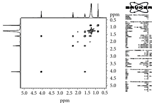
FIGURE 6: COSY spectrum of PEN 4 .
