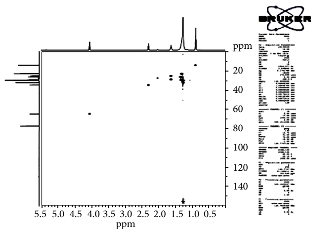
FIGURE 4: HSQC spectrum (CDCl 3 , 125 MHz) of PEN 4 .
