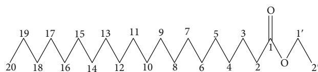
FIGURE 7: Ethyl arachidate or arachic acid ethyl ester (AAEE) structure.
