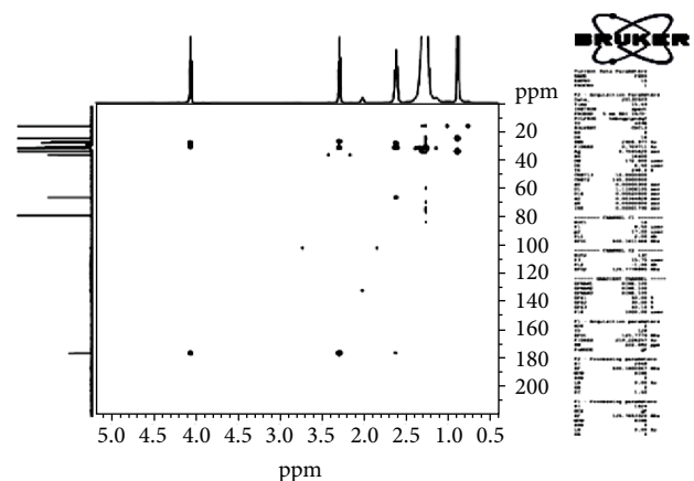
FIGURE 5: HMBC spectrum (CDCl 3 , 125 MHz) of PEN 4 .
