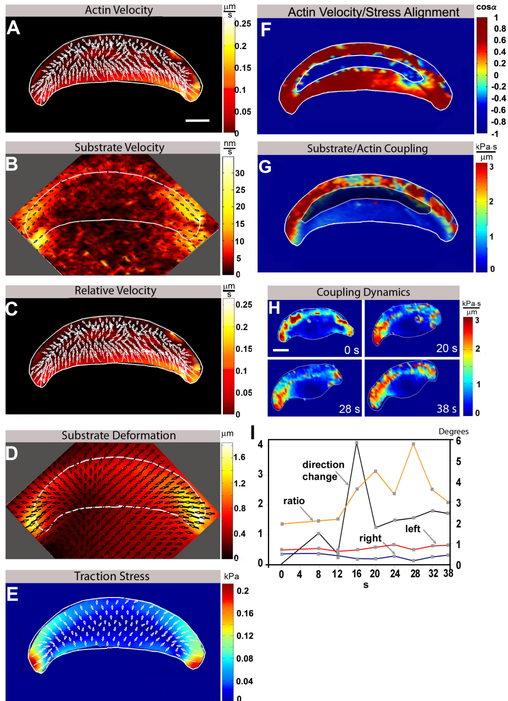
Figure 2. Comparative mapping of actin velocity and substrate stress and computation of the adhesion strength parameter. (A–C) Actin velocity map (A) minus substrate velocity map (B) gives the map of actin velocity with respect to the substrate (C). (D and E) A substrate deformation map (D) was used to calculate the stress map (E). (A–E) Arrows indicate the direction and relative magnitude of velocity (A–C), deformation (D), and traction stress (E). (F) Map of actin velocity–stress alignment and cosine of the angle between F-actin velocity and stress vectors. (G) A map of adhesion strength was computed as a ratio of the stress map and the map of actin velocity with respect to the substrate. The contour within the cell corresponds to the region of the opposite alignment of actin velocity and stress, which is shown in blue in F. (H) The analysis of adhesion strength dynamics in a cell that changed direction of motion showed a drop in adhesion strength upon detachment at one side of the cell (at 20 s) and its subsequent recovery (Video 2). (A–H) The cell margin is shown with the white outline. (I) Coupling in 120\text{-}\mu\text{m}^2 areas (approximately one quarter of the cell) at the two sides of the cell shown in H was quantified as a fraction of the area in which coupling exceeded 1\text{ kPa}\cdot\text{s}/\mu\text{m} . Resulting values for the left and right sides and their ratio (left to right) are plotted (left, right, and ratio are measured in nondimensional units on the left scale) versus time along with the cell turn angle (direction change is measured in degrees on the right scale). Cell turn angle was measured as the difference between the orientations of the cell’s long axis (determined by approximating the cell with an ellipse) in each pair of the sequential frames. Time is indicated in the images. Bars, 10\text{ }\mu\text{m} .
