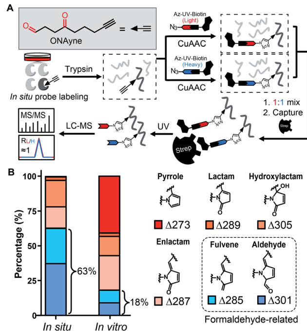
Fig. 2 Adduct profile and proteome-wide selectivity of the \gamma -dicarbonyl probe ONAyne. (A) Chemical structure of ONAyne and schematic workflow for identifying ONAyne-adducted sites across the proteome. (B) Bar chart showing the distribution of six types of ONAyne-derived modifications formed in situ and in vitro (note: before probe labelling, small molecules in cell lysates were filtered out through desalting columns).
