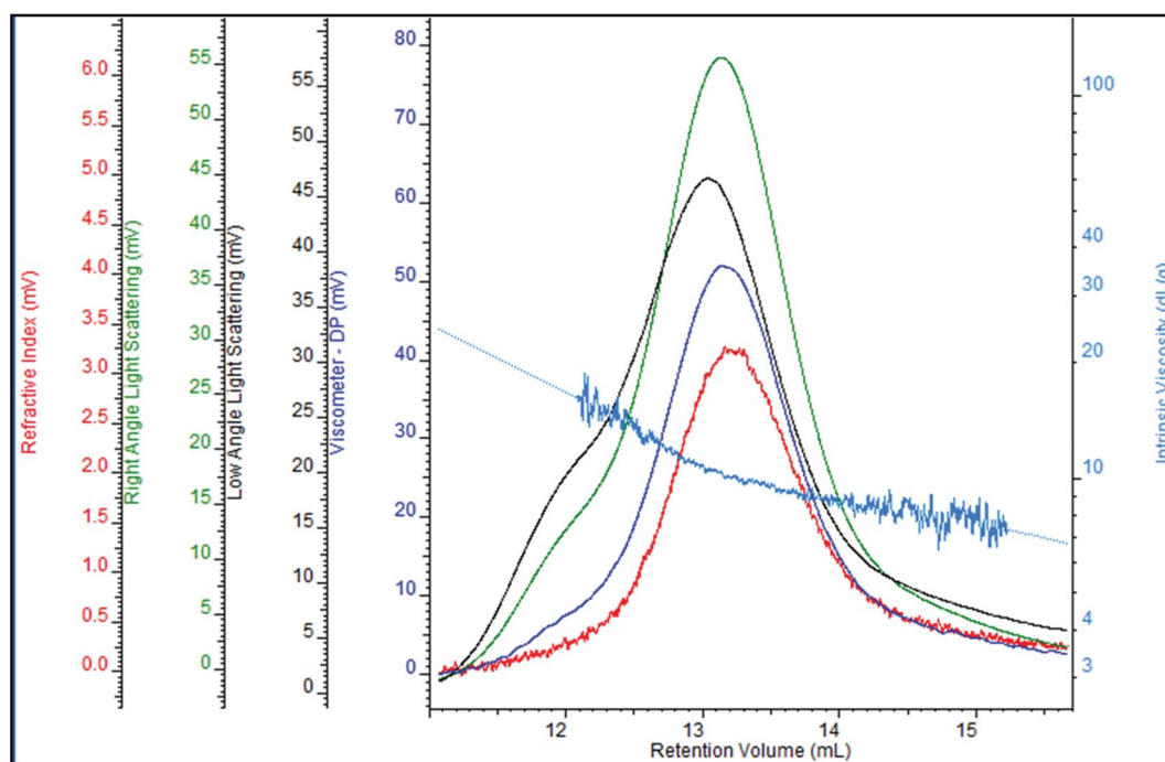
Fig. 4 Distribution of molecular weight and molecular viscosity of EPS produced by S. pararoseus JD-2.
