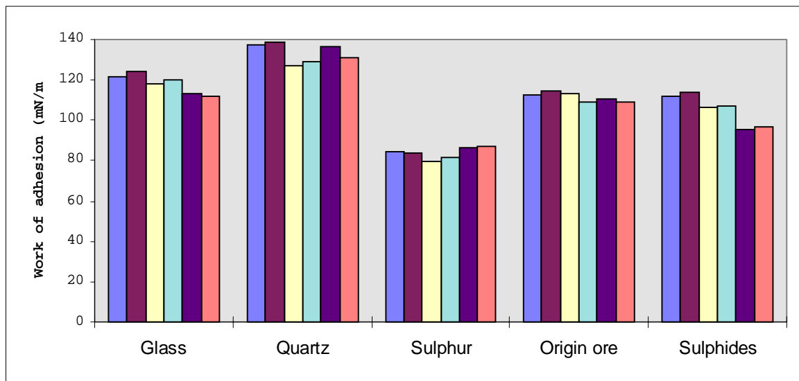
Fig. 6. The results of work of adhesion obtained for water on different surfaces (calculated from six measurements for each surface)
