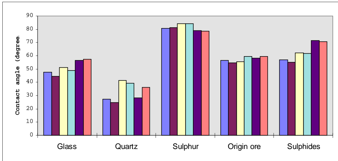
Fig. 5. Contact angle for water on different surfaces (six measurements for each surface)
