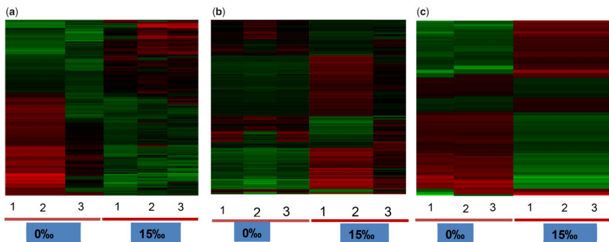
Fig. 1. —Heatmap showing differential expression pattern of transcripts at 0‰ and 15‰ salinities for three different Macrobrachium species. (a) M. australiense (876 transcripts), (b) M. tolmerum (861 transcripts), and (c) M. novaehollandiae (925 transcripts).
