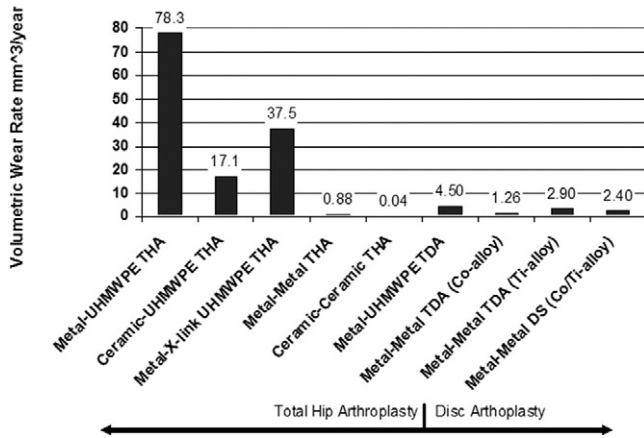
Fig. 2. A graphical comparison of data showing the amount of wear debris generated from different types of total joint arthroplasties demonstrating that there is relatively less (10 \times ) polymeric debris generated by a total disc arthroplasty with a metal-on-polymer articulation. However, this difference is not apparent with metal-on-metal articulating implants. Note: Figure References: Metal-Poly:24 Ceramic-Poly:25, Metal-X-linked Poly: 22 Metal-X-linked Poly: 26, Metal-X-linked Poly: 27, Metal-X-linked Poly: 28, Metal-Metal: 29, Ceramic-Ceramic: 30, Metal-UHMWPE TDA: 17, Metal-Metal TDA: 18.
