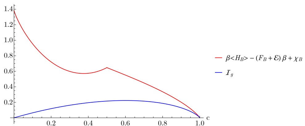
Figure 2. Plots of the information gain \mathcal{I}_g and the right hand side of Equation (27) as a function of c .
