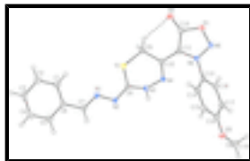
Fig. 1. The asymmetric unit of the title compound, showing 30% probability displacement ellipsoids. The intramolecular hydrogen bond is shown as a dashed line.
