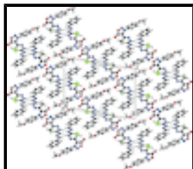
Fig. 2. The crystal packing of the title compound viewed along the a axis. Intermolecular hydrogen bonds are shown as dashed lines.
