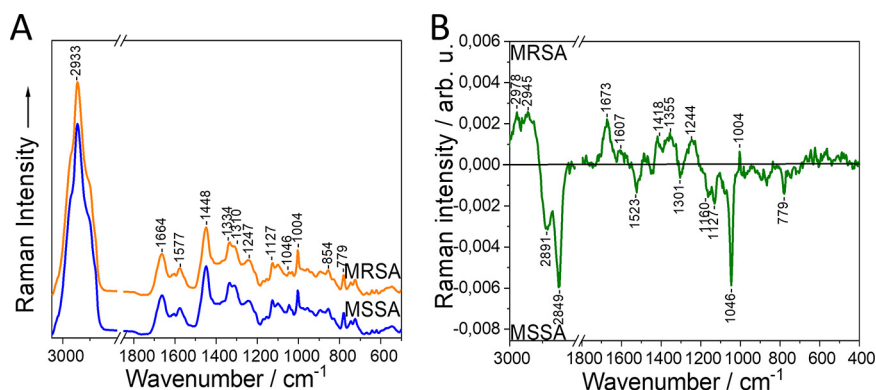
FIG 3 Mean Raman spectrum (A) and difference spectrum (B) of MRSA and MSSA strains by using single-cell analysis with 532 nm excitation. arb. u, arbitrary units. Spectra are shifted vertically for clarity.
