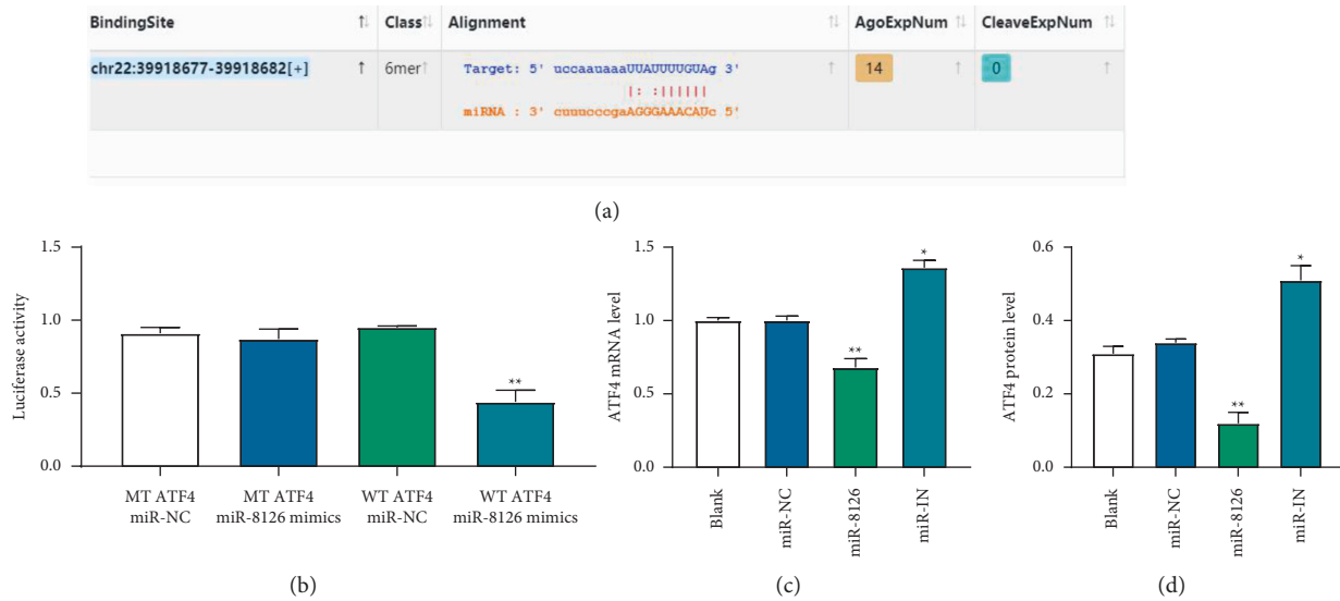
FIGURE 7: miR-8126 promotes rat hippocampal neuron viability by targeting ATF4. Target scan predicts miR-8126 and ATF4 binding sequence (a); miR-8126 binds to ATF4 mRNA and inhibits its activity by dual luciferase report assay (b); qRT-PCR (c); and Western blot (d). All * P < 0.05 and ** P < 0.01 .
