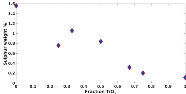
Fig. 9 Impact of increasing fraction of TiO 2 on approximated sulphur weight% from SEM/EDX.
