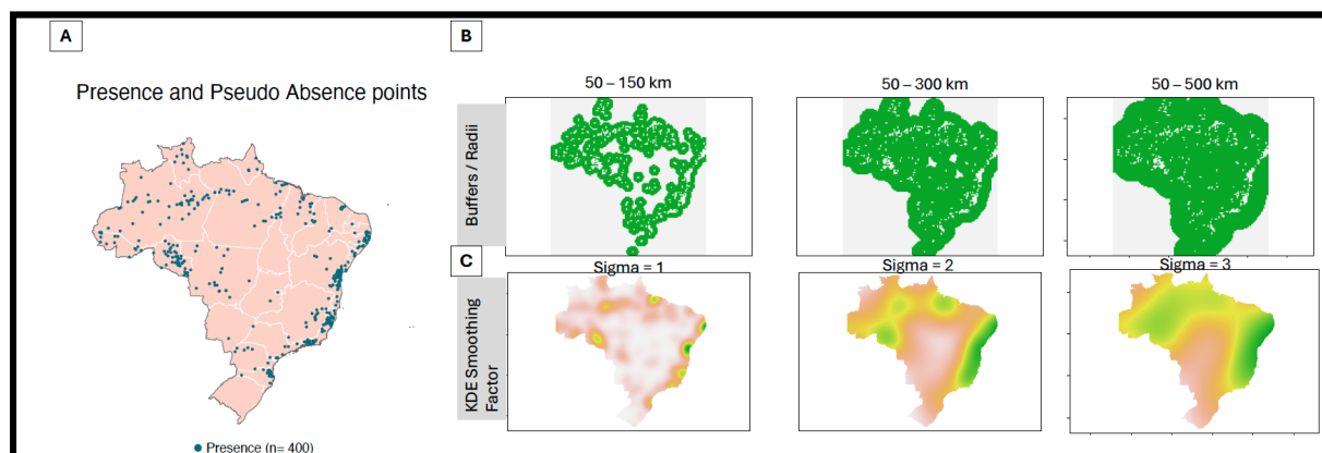
Figure S3 Illustration of spatial distribution of presence and pseudo-absence points used for modeling.
