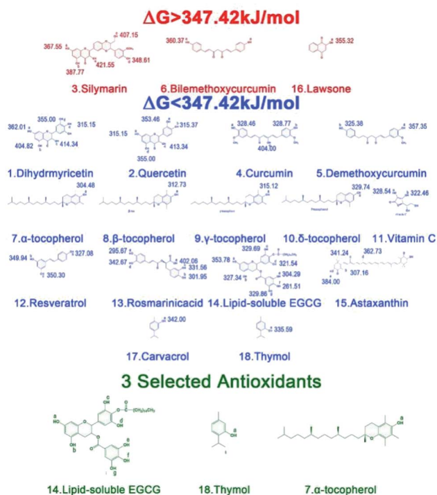
Fig. 4 Screening process of natural phenolic antioxidants and the \Delta G ( \text{kJ mol}^{-1} ) of \text{ArO-H} bonds at different position are indicated in the structures.
