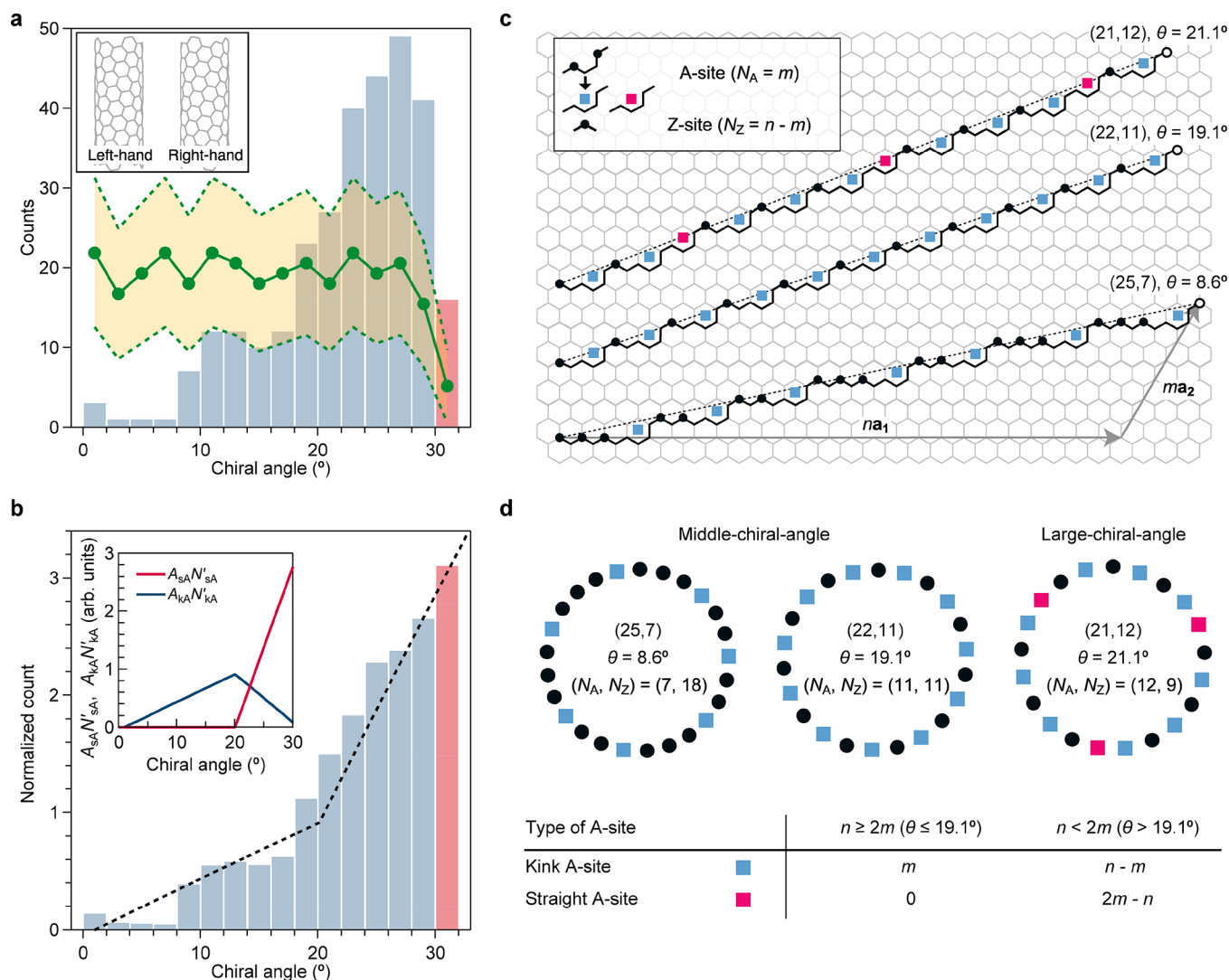
Figure 3. Chiral angle dependence of structure distribution. (a) Histogram of SWCNTs with diameters of 1.70–2.74 nm as a function of the chiral angle. Bin size, 2^{\circ} . The red bar at 30^{\circ} represents the number of armchair SWCNTs with the same bin size. Green markers show the number of SWCNTs expected under the random growth condition with 95% confidence interval estimated from the Poisson distribution (orange band). The inset shows an example of enantiomers of the (8,4) SWCNT. (b) Histogram of the normalized count. The black dotted line represents the fitting result. The inset shows the growth contributed to by straight armchair sites (A-sites; A_{SA}N'_{SA} ) and kink A-sites ( A_{KA}N'_{KA} ). (c) Open tube edges of (25,7), (22,11), and (21,12) SWCNTs projected onto graphene plane (solid black lines). Dotted lines represent open tube edges with the minimal circle length. As shown in the inset, red and blue squares and black circles indicate A-sites and zigzag sites (Z-sites), respectively, and their numbers are indicated by N_A and N_Z . (d) Open tube edges represented using A-sites and Z-sites (upper panel). Summary of the number of consecutive and isolated A-sites for a ( n,m ) SWCNT (bottom panel).
