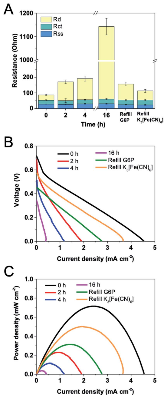
Fig. 6 Variations of (A) internal resistances, (B) open circuit voltages and (C) power densities versus current density for an EFC operated for 16 h at a constant load of 50\ \Omega .
