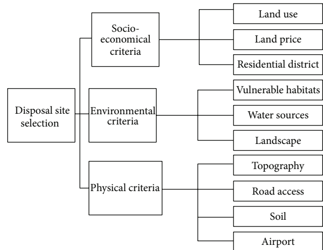
FIGURE 1: Hierarchical structure for disposal site selection problem.
