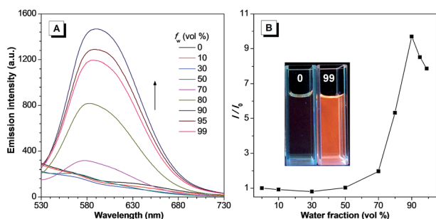
Fig. 1 (A) Emission spectra of TPEQN-P (10 \mu M) in a DMSO/water mixture with different water fractions ( f_w ). (B) Plot of emission intensity at 590 nm versus the composition of the water mixtures of TPEQN-P, where I_0 is the emission intensity at 590 nm of TPEQN-P in pure DMSO solution. Inset: photograph of TPEQN-P in DMSO/water mixture with 0 and 99% f_w under 365 nm irradiation.
