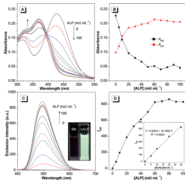
Fig. 2 (A) UV-vis and (C) emission spectra of TPEQN-P (10 \mu M) after addition of ALP with different concentrations. Plots of (B) absorbance at 430 nm and 370 nm and (D) emission intensity at 495 nm, vs. the concentration of ALP. Inset in (C): photograph of TPEQN-P in the absence and presence of ALP under 365 nm irradiation. Inset in (D): the linear relationship between intensity at 495 nm and the concentration of ALP (0–30 mU mL -1 ).
