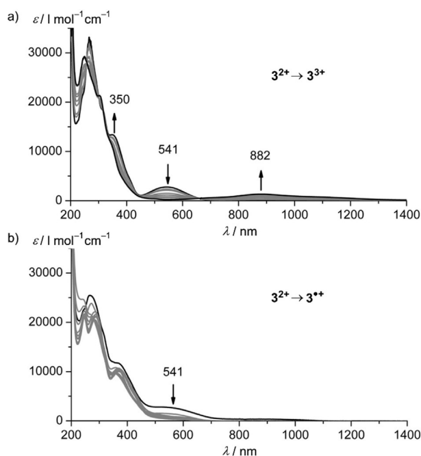
Figure 3. UV/Vis/NIR absorption spectra of 3[PF_6]_2 in acetonitrile with 0.1 M [ n Bu 4 N][PF 6 ] at 298 K collected during a) electrochemical oxidation and b) electrochemical reduction.
