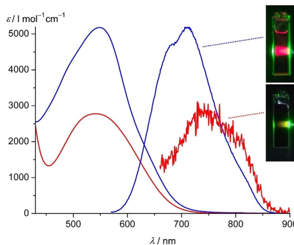
Figure 4. UV/Vis/NIR absorption and emission spectra (scaled to the respective MLCT absorption band) of 2[PF_6]_2 (blue) and 3[PF_6]_2 (red) in acetonitrile at 298 K ( \lambda_{exc} = 544 nm). The photos display cuvettes of acetonitrile solutions of 2[PF_6]_2 and 3[PF_6]_2 under irradiation with green light (560 nm).
