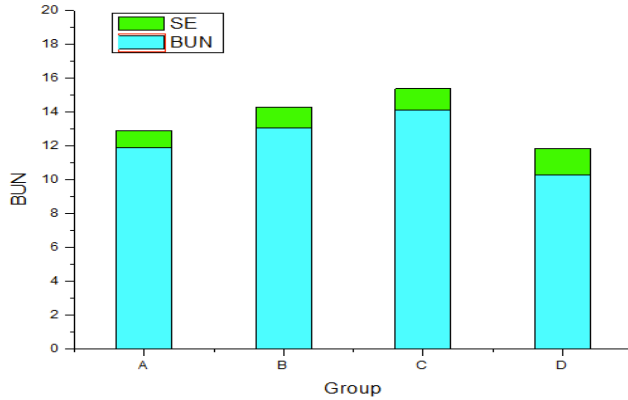
Fig. (1). The mice BUN test results for each group after the test.
