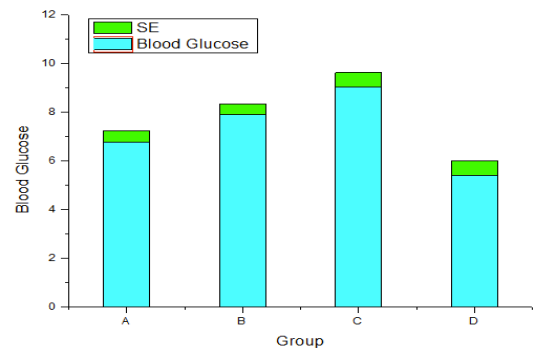
Fig. (3). The mice blood glucose test results for each group after the test.
