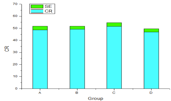
Fig. (2). The mice CR test results for each group after the test.
