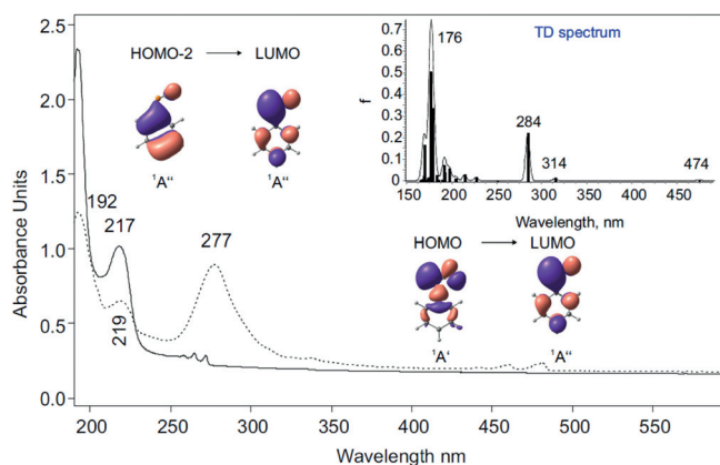
Figure 2. Solid: UV/Vis spectrum of 3 isolated at 10 K in Ar. Dashed: UV/Vis spectrum of 1 at 10 K; the photochemistry of 3 after irradiation at λ = 254 nm in Ar at 10 K. Inset: Computed TD-B3LYP/6–311++G(3df,3pd) spectrum of 1 .
