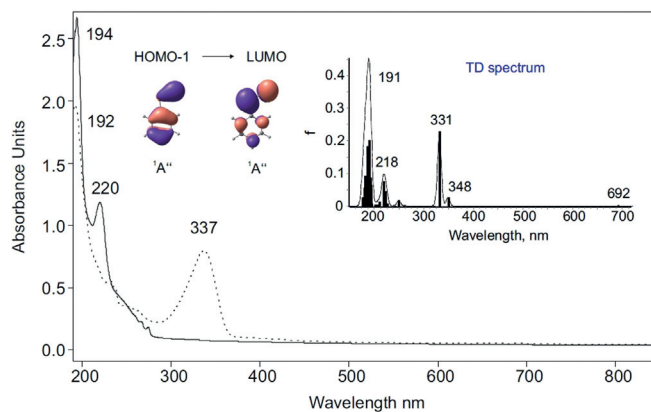
Figure 4. Solid: UV/Vis spectrum of 4 isolated at 10 K in Ar. Dashed: UV/Vis spectrum of 2 at 10 K; the photochemistry of 4 after irradiation at \lambda = 254 nm in Ar at 10 K.
