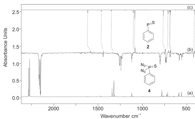
Figure 3. a) IR spectrum of 4 computed at B3LYP/6-311++G(3df,3pd) (unscaled). b) IR difference spectra showing the photochemistry of 4 after irradiation at \lambda = 254 nm in argon at 10 K. Downward bands assigned to 4 disappear while upward bands assigned to 2 appear after 15 min irradiation time. c) IR spectrum of 2 computed at B3LYP/6-311++G(3df,3pd) (unscaled).
