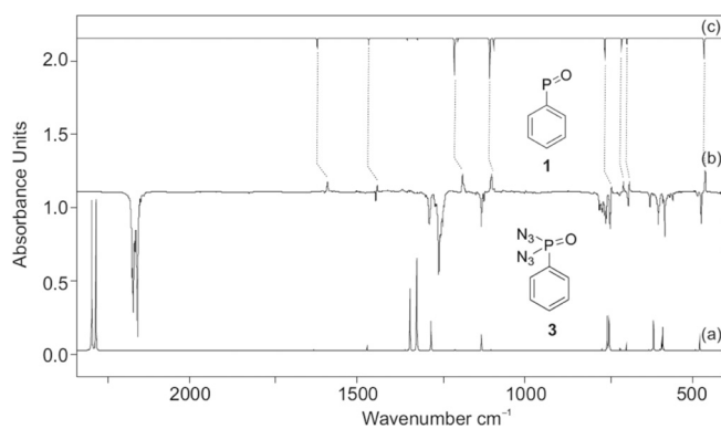
Figure 1. a) IR spectrum of 3 computed at B3LYP/6–311++G(3df,3pd) (unscaled). b) IR difference spectra showing the photochemistry of 3 after irradiation at λ = 254 nm in argon at 10 K. Downward bands assigned to 3 disappear while upward bands assigned to 1 appear after 15 min irradiation time. c) IR spectrum of 1 computed at B3LYP/6–311++G(3df,3pd) (unscaled).
