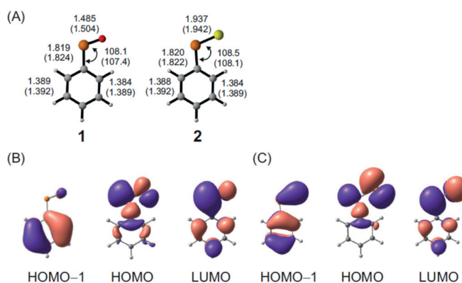
Figure 5. A) Selected bond lengths [Å] and angles [°] of 1 and 2 at B3LYP/6-311++G(3df,3pd). The values in parentheses were computed at MP2/cc-pVTZ; (B), C) Molecular orbitals of 1 (B) and 2 (C) at B3LYP/6-311++G(3df,3pd).
