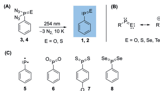
Scheme 1. A) Photochemical generation of 1 and 2 . B) Resonance structures of the phosphinidene chalcogenides. C) Triplet phosphinidene ( 5 ), phenyldioxophosphorane ( 6 ), and previously prepared heavier congeners of 6 , namely 7 and 8 .
