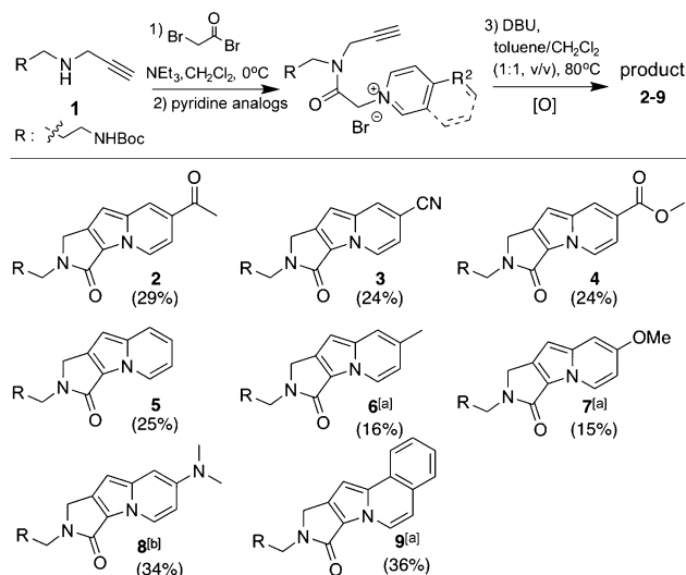
Scheme 2. Synthesis of lactam-embedded indolizine core structures. The yields given are for the isolated product after four steps. [a] \text{Ag}_2\text{O} was used to catalyze the 1,3-dipolar cycloaddition. [b] [\text{AuPPh}_3\text{Cl}] was used as a catalyst; DDQ was added for the oxidative aromatization. Boc = tert -butoxycarbonyl.
