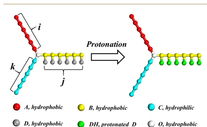
Fig. 1 Schematic illustration of the miktoarm star polymer \mu\text{-A}_i(\text{B}(\text{D}))_j\text{C}_k with a pH-responsive arm. White, red, yellow, cyan, gray and green represent O, A, B, C, D and DH beads, respectively. The meaning of colors in this figure is suitable for all figures in this paper.
