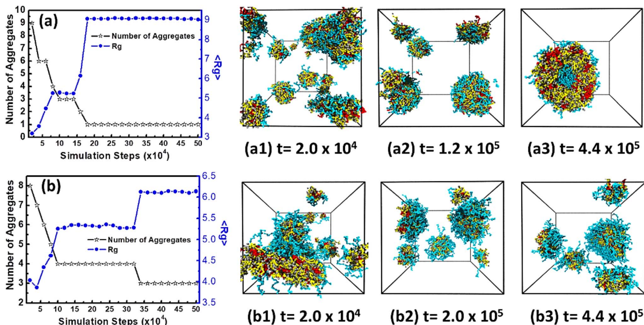
Fig. 4 The variations of number of aggregates and mean gyration radius ( R_g ) with simulation step and the corresponding dynamic evolution: (a) vesicle formed at arm lengths at j = 15 and k = 5 ; (b) spherical micelle formed at arm lengths at j = 20 and k = 15 . Solvents and beads O are omitted for clarity.
