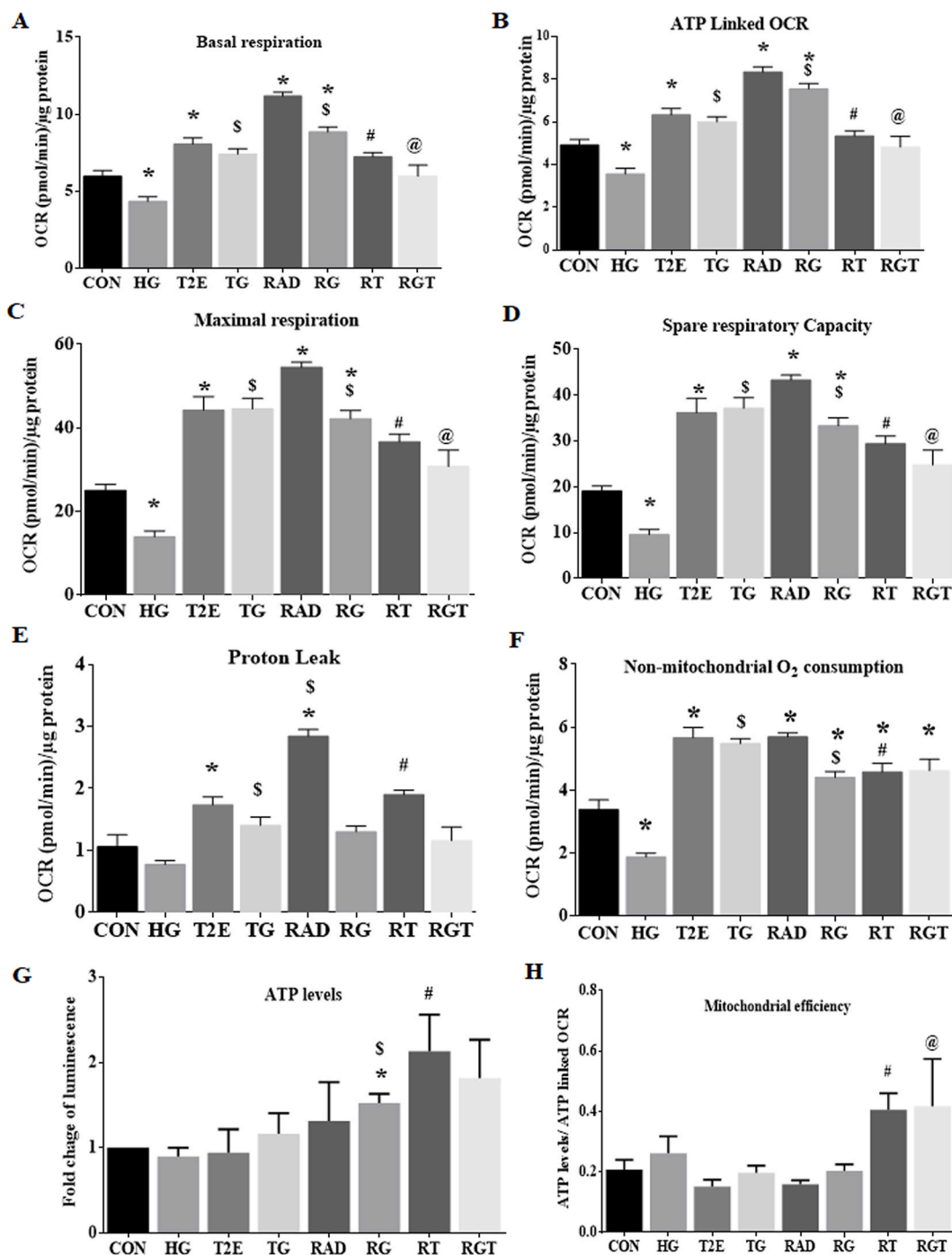
Fig. 3. MnTE-2-PyP increased mitochondrial ATP synthesis efficiency after radiation and hyperglycemia stress in normal prostate fibroblasts. Human prostate fibroblast cells were treated with 20 mM glucose (HG) and 30 μM MnTE-2-PyP (T2E) followed by 3 Gy of X-rays (RAD). Cells were subjected to Seahorse bio-analyzer to measure mitochondrial oxygen consumption rate (OCR). A. Basal respiration, B. ATP linked OCR, C. Maximal respiration, D. Spare respiratory capacity, E. Proton leak linked OCR and F. Non-mitochondrial OCR were measured. G. Total levels of ATP were measured in human prostate fibroblasts after 5 days of radiation. H. ATP levels were normalized by average value of ATP linked OCR (Fig. 3B). Levels of ATP produced using per unit of ATP linked OCR were measured. All graphs are representative of at least 3 independent experiments.
