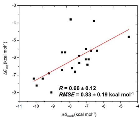
Fig. 1 Correlation between molecular docking and experiment. The calculated errors are the standard error.
