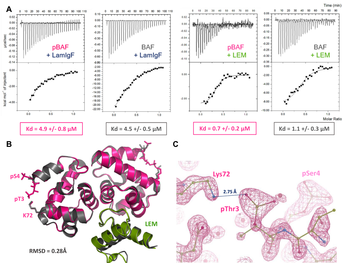
Figure 7. pBAF still forms a ternary complex with both lamin A/C and emerin. (A) ITC analysis of the interactions between pBAF and the lamin LamIgF or the emerin LEM fragments. pBAF (or BAF for comparison) being in the cell, the fragment LamIgF or LEM was injected and the heat signal was measured as a function of the injection number. Experiments were performed in duplicate, as detailed in Supplementary Table S2. (B) X-ray structure of pBAF bound to the LEM domain of emerin. The 3D structure of the complex is displayed as a cartoon, pBAF being in pink and the LEM domain in green. It is superimposed with that of BAF bound to the LEM domain (in grey; PDB 6GHD; (29)). The side chains of residues Thr3, Ser4 and Lys72 are displayed in sticks in both complexes. The specified RMSD value was calculated between all atoms of the pBAF-LEM and BAF-LEM complexes. The statistics of the pBAF-LEM structure are presented in Supplementary Table S1. (C) Zoom view on the electron density map defining the position of the side chains of pThr3, pSer4 and Lys72 in pBAF.
