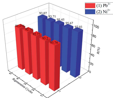
Fig. 14 Removal efficiency of five adsorption–desorption cycles of regenerating Fe 3 O 4 @SiO 2 -g-PAMAM-AO on Pb(II) and Ni(II). (C 0 = 50 mg L -1 , T = 298 K, pH (Pb 2+ ) = 5.5, pH (Ni 2+ ) = 8, t = 2 h).
