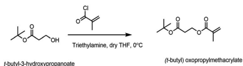
Fig. 2 Synthesis of propionate monomer from t -butyl-3-hydroxypropanoate.
