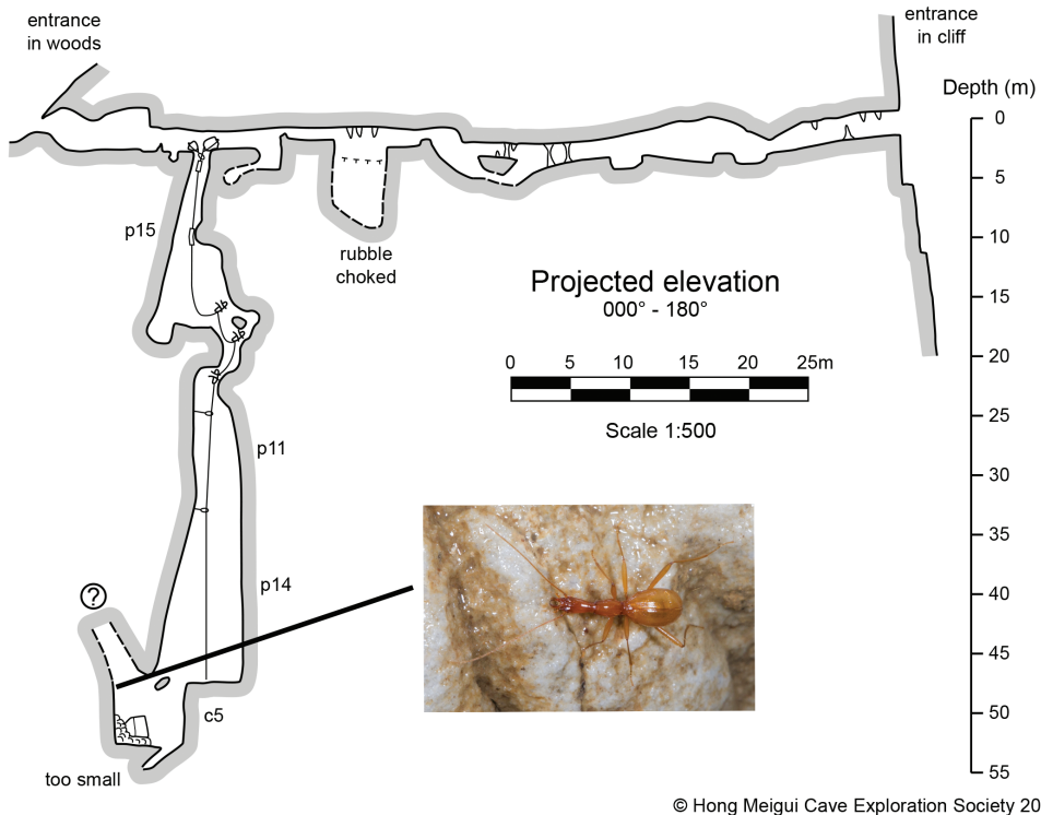
Figure 4. Map of Qiankou Dong, to show where the holotype of Wulongius qilinger gen. nov. and sp. nov. was discovered) (courtesy of Prof. Yuanhai Zhang and Hong Meigui Cave Exploration Society).
