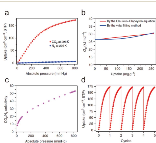
Fig. 34 (a) The CO 2 and N 2 adsorption isotherms for FJI-H14 at 298 K. (b) The isosteric heat of CO 2 adsorption ( Q_{st} ) for FJI-H14. (c) The IAST selectivity of FJI-H14 for CO 2 /N 2 (15:85). (d) 5 Cycles of CO 2 adsorption for FJI-H14 at 298 K. Reproduced from ref. 136 with permission from Springer Nature, Copyright 2017.
