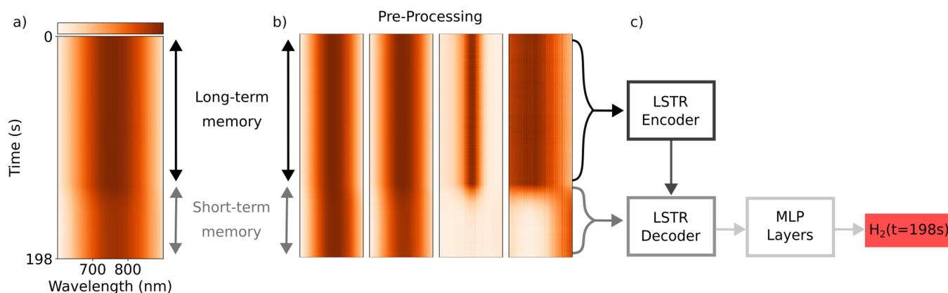
Figure 2. Long Short-term Transformer Ensemble Model for Accelerated Sensing (LEMAS). Illustration of the deep learning model used in this work based on the LSTR architecture (see Figure S16 for a more detailed illustration of the LSTR model). (a) The input data to the model consist of a time sequence of the past evolution of the spectral response of the sensor. In this figure the time sequence consists of 600 time steps corresponding to 198 s. (b) The time sequence is first split into long- and short-term memory and preprocessed using four different methods, including wavelength dependent min-max normalization, standard normal variate standardization, and level scaling, before the concatenation of the preprocessed data is being fed to the LSTR. (c) The LSTR first compresses the long-term memory to a fixed length latent representation in the LSTR encoder. Second, the LSTR decoder extracts relevant temporal features in the short term memory while also querying the compressed long-term memory. The extracted temporal features are then passed through a stack of multilayer perceptron (MLP) layers to obtain a prediction of the current H_2 concentration.
