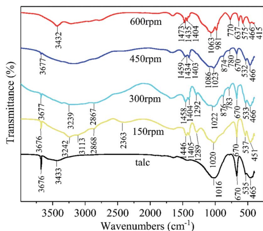
Fig. 5 FT-IR patterns of talc, the milled products at 150 rpm, 300 rpm 450 rpm and 600 rpm (60 min milling time).
