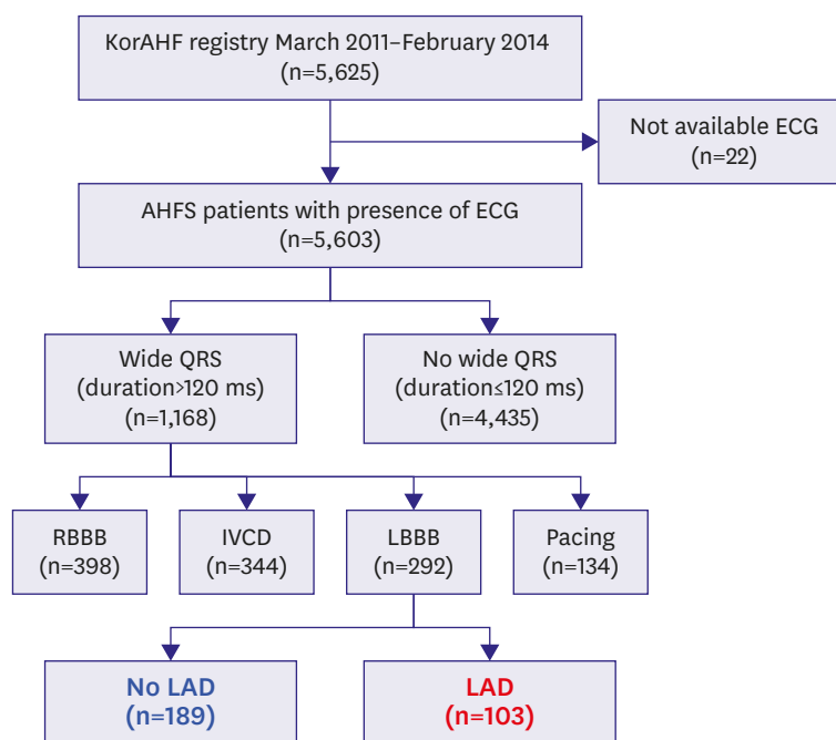
Figure 1. Study flow.
